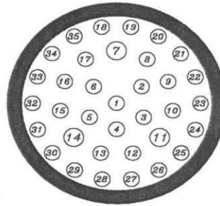
PLUG ( SOCKET )
